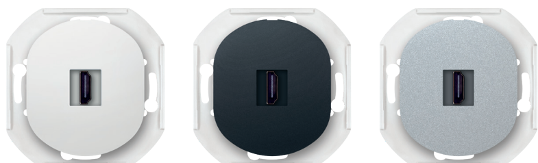
E6163.x Priključnica HDMI/HDMI Keystone HDMI/HDMI socket Keystone • Za konekciju kablova za prenos signala preko HDMI priključka • For the transmission of signal through HDMI connector
