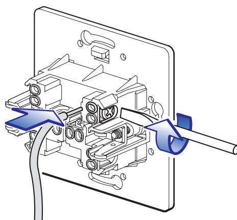
VIJČANA MONTAŽA INSTALLATION WITH SCREWS
